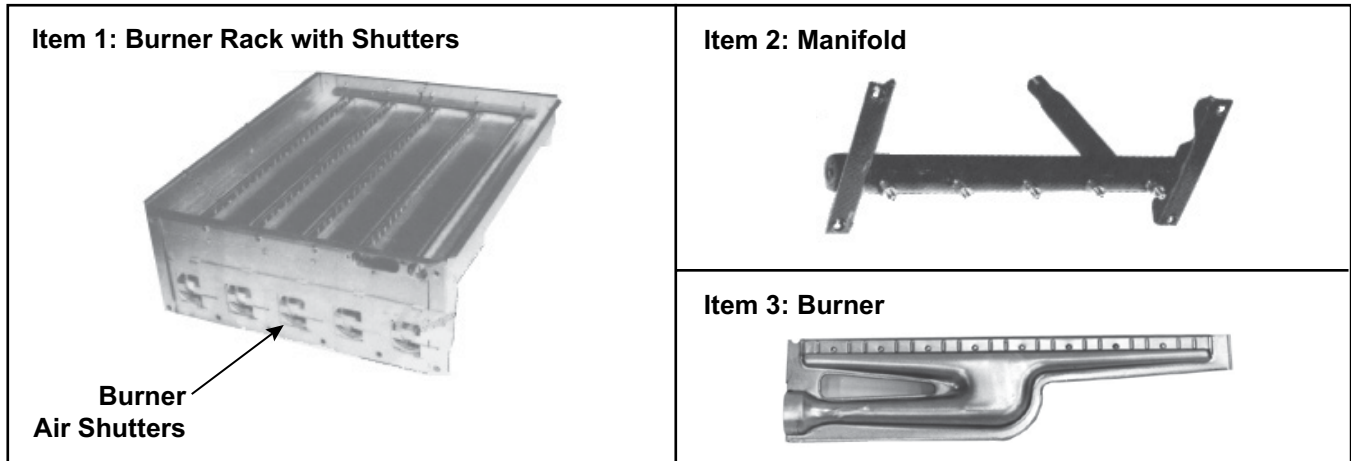
Figure 8. Burner Components (Refer to Table 11)
